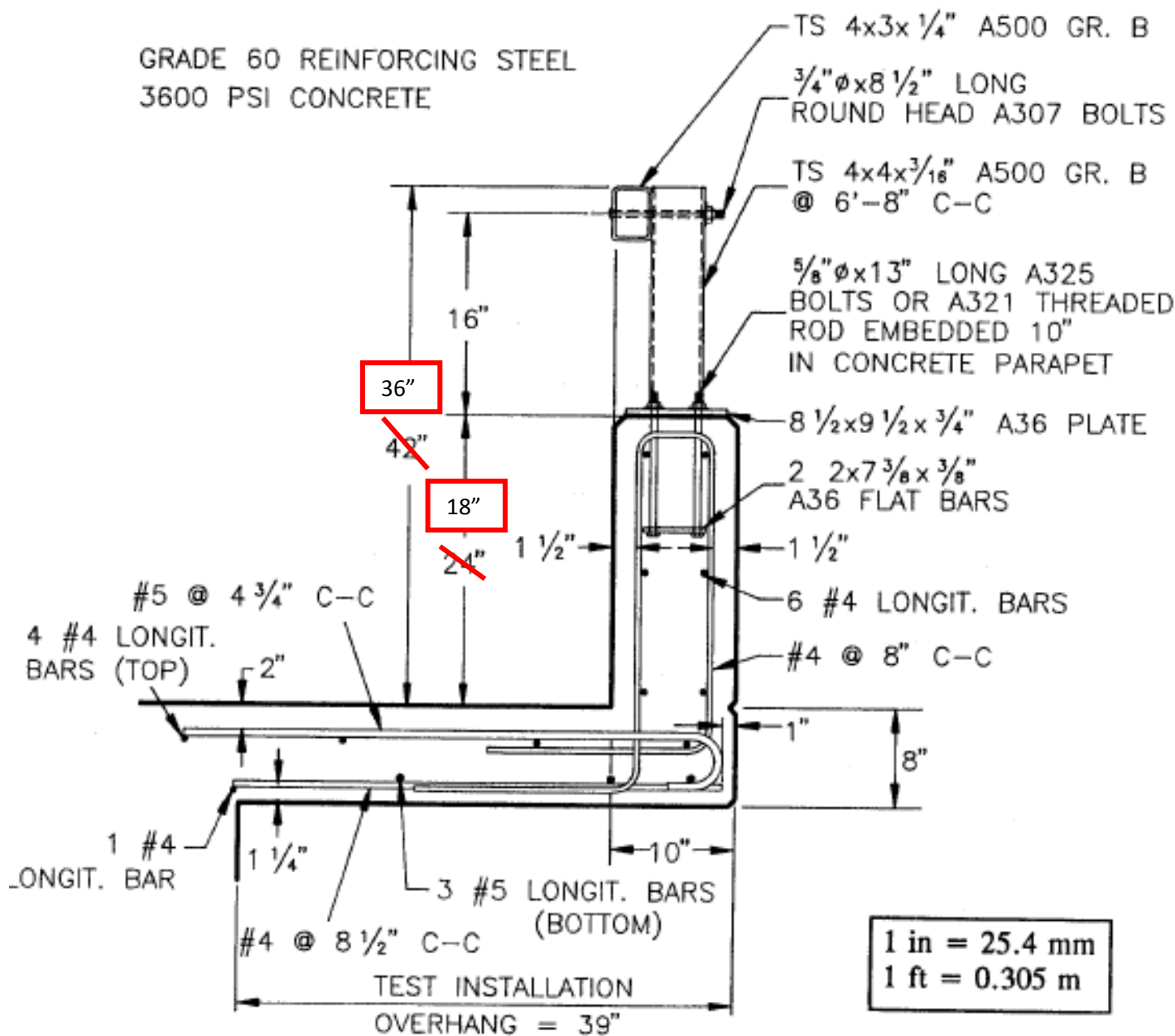
Figure B7.29. BR27C Flush Mounted Bridge Railing (8,40,42).
